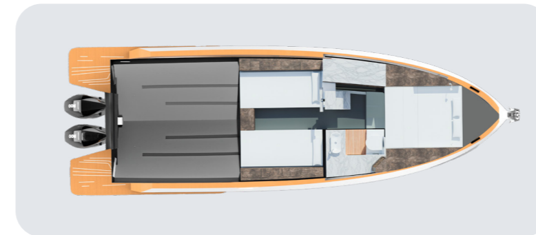
Outboard interior layout
